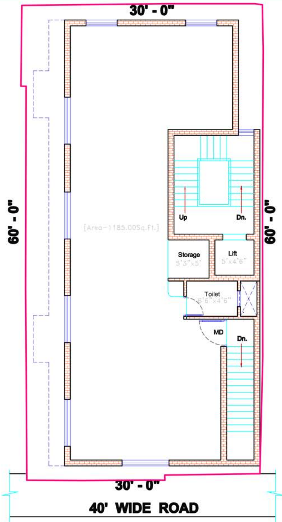
SITE CUM FIRST FLOOR PLAN
