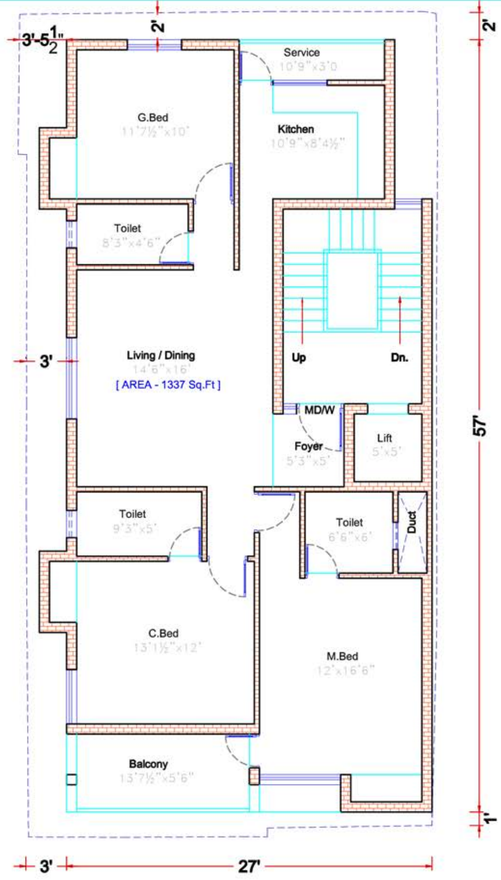
TYPICAL FLOOR PLAN SECOND AND THIRD
