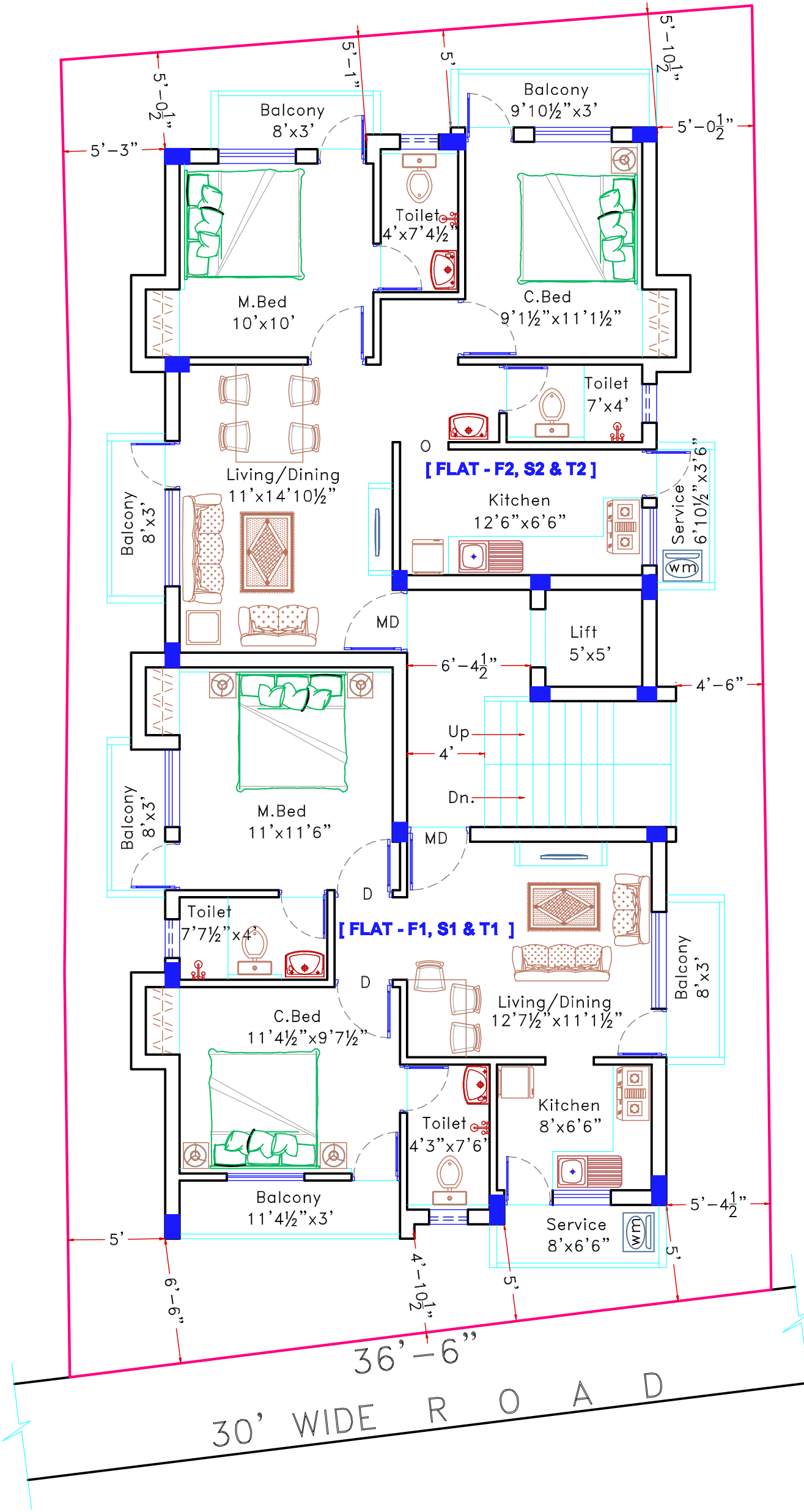
TYPICAL FLOOR PLAN [ FIRST, SECOND & THIRD ]
